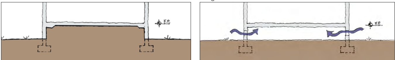
FIGURE 11 ALTERNATIVES TO FOUNDATIONS ON FILL
