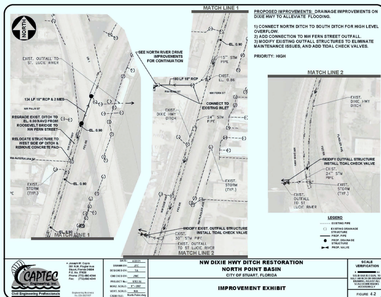
Figure 4.2 NW Dixie Highway Ditch Restoration
