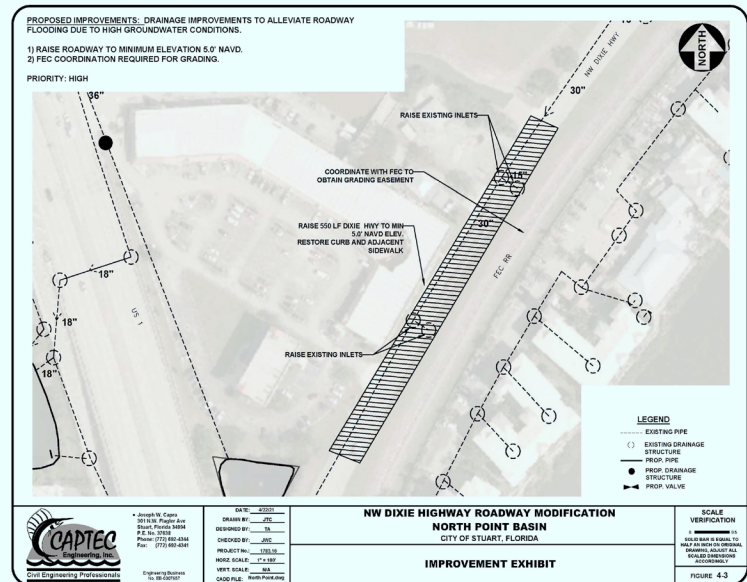
Figure 4.3 NW Dixie Highway Roadway Modification
