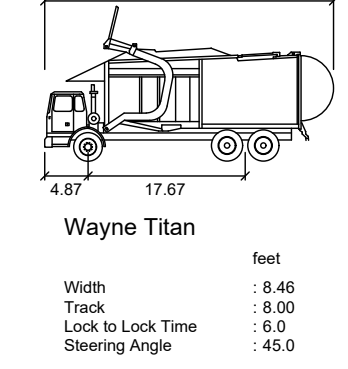
DUMPSTER TRUCK DETAIL
