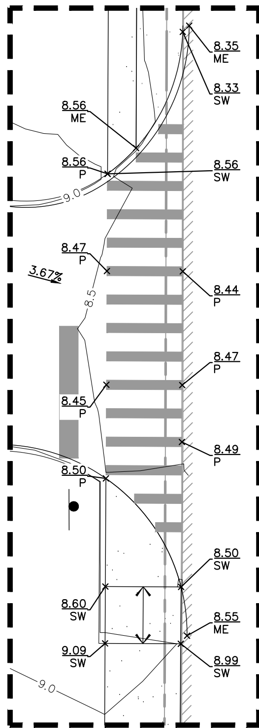
CROSSWALK DETAIL
