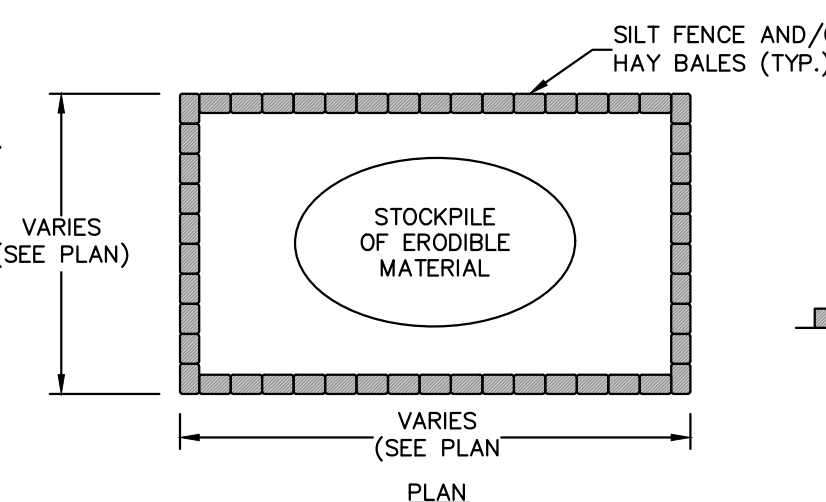
SEDIMENT CONTROL FOR STOCKPILING OF ERODIBLE MATERIAL N.T.S.
