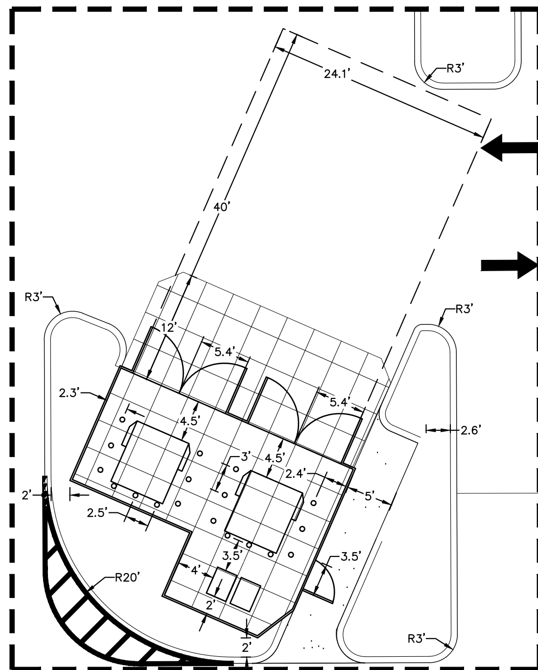
SCALE 1" = 10'
