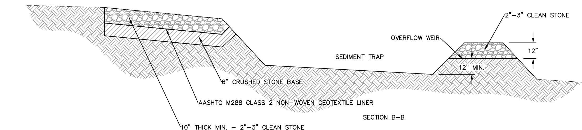
CONSTRUCTION EXIT N.T.S.
