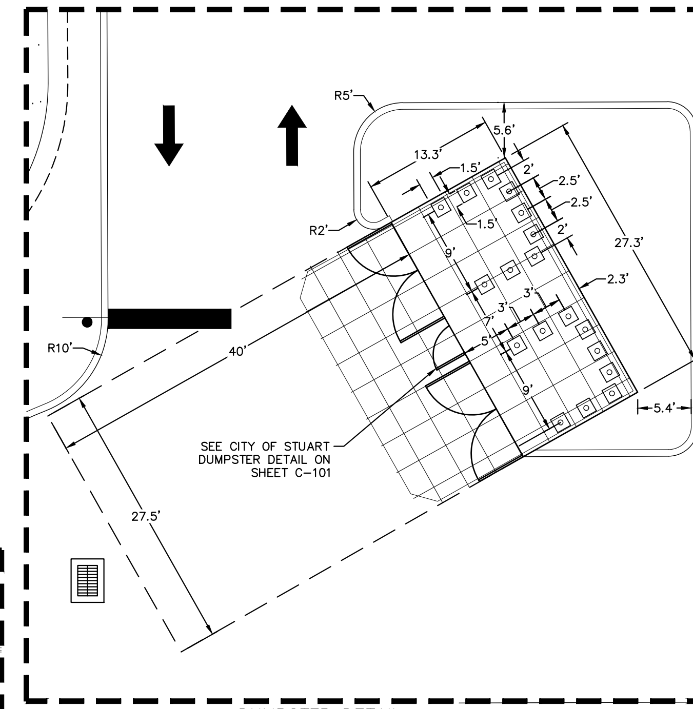
DUMPSTER DETAIL
